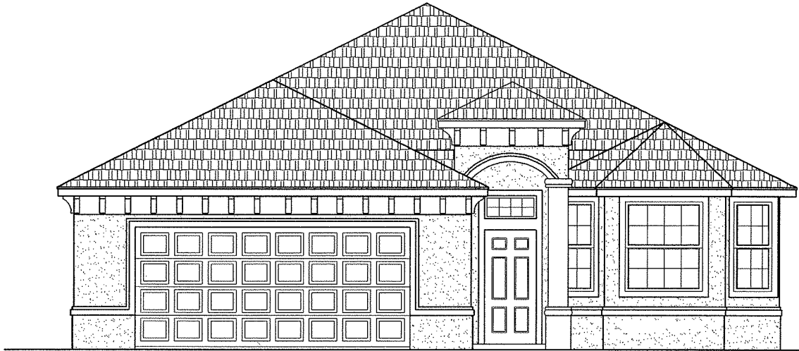
FRONT ELEVATION A
